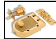
Deadlocks
